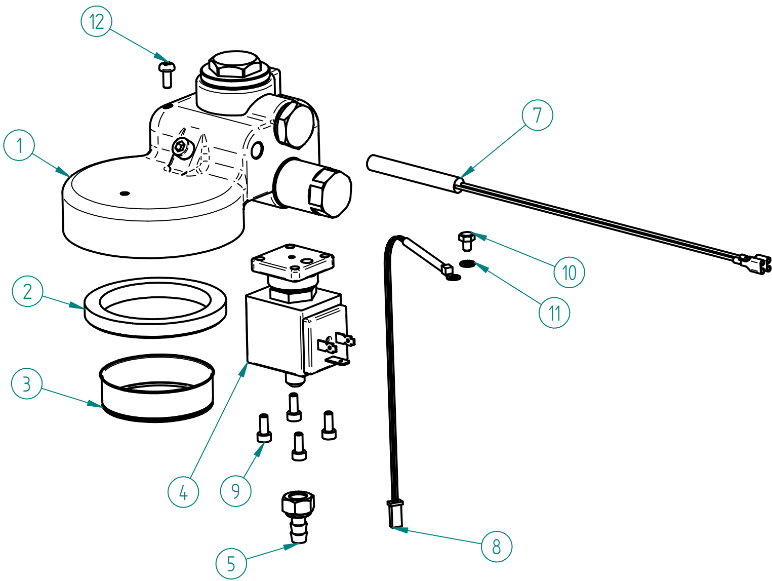
60 - 7.0.028.1153 - GRUPO ECC-07 C/ RESIST. CONJ. 60 - ECC-07 GROUP W/ RESIST.
